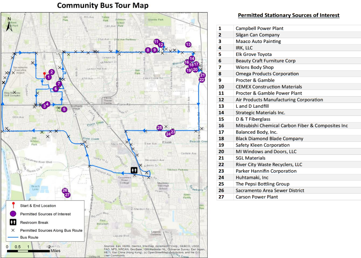
Figure 3-3 Bus tour route map with key permitted sources of interest along the route highlighted.
