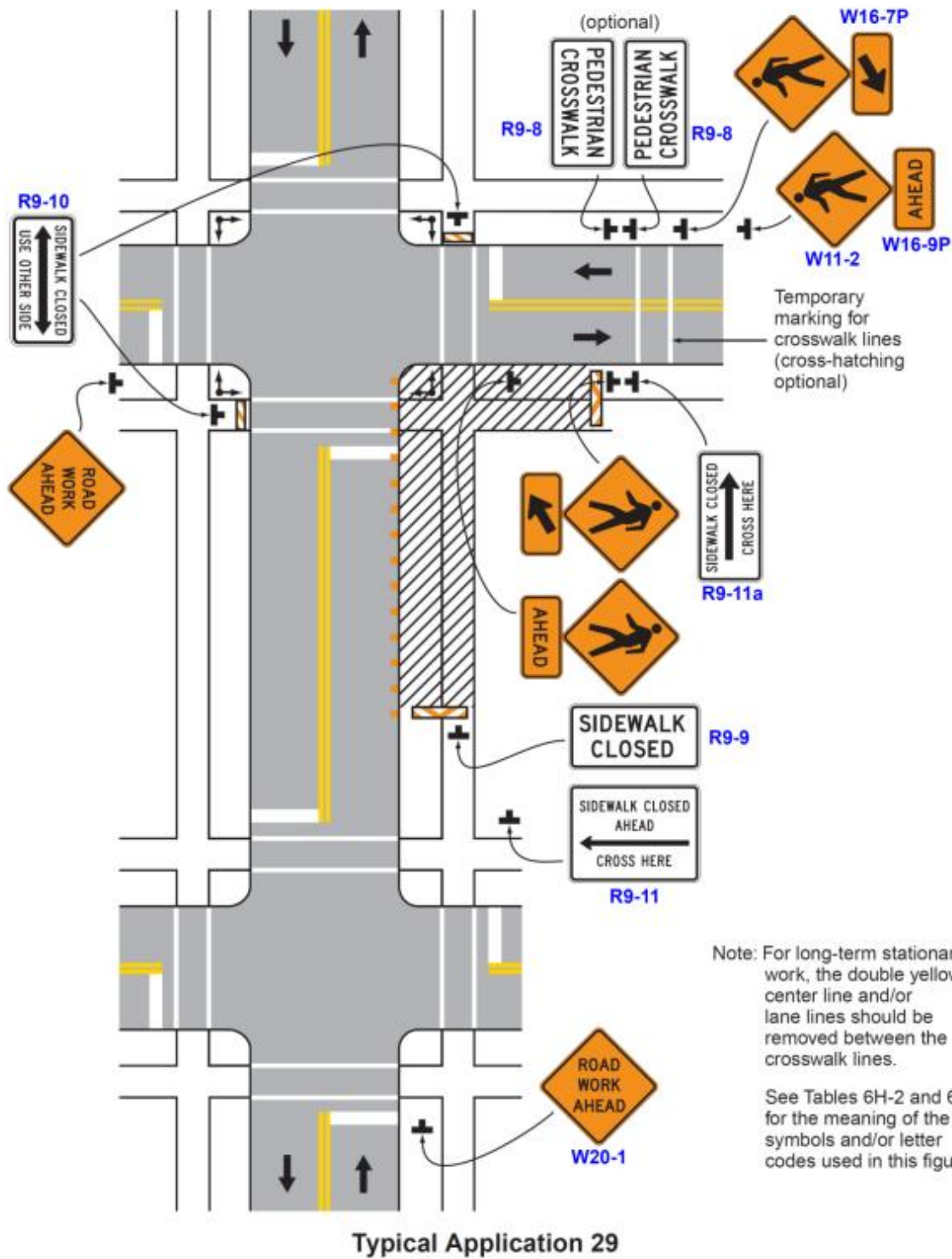
Figure 13: Crosswalk Closures and Pedestrian Detours (Figure 6H-29 from California Manual on Uniform Traffic Control Devices)
