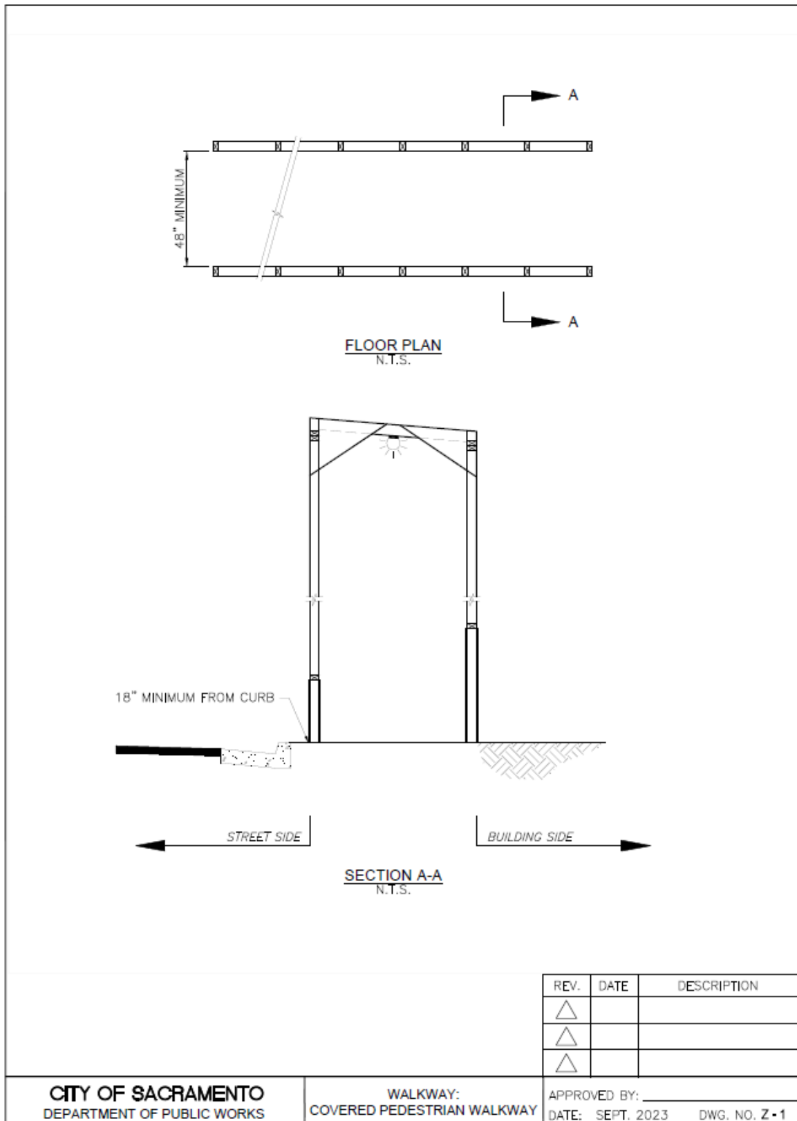
Figure 12: Walkway: Covered Pedestrian Walkway
